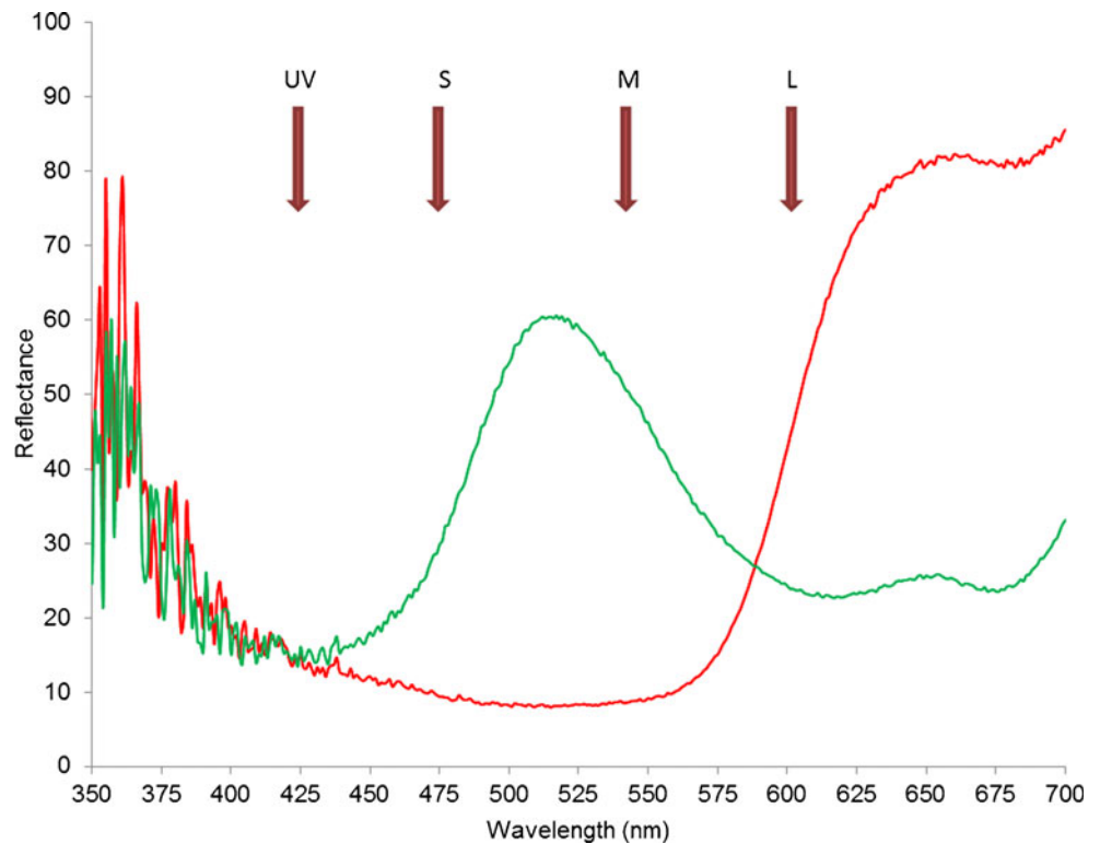
Fig. 2 Spectral reflectance functions of the red and green backgrounds used in the experiment. The arrows denote the peak sensitivity wavelengths of the four receptors ( UV , S , M , and L ) in the chicks' color-vision system, as reported by Osorio et al. (1999)
